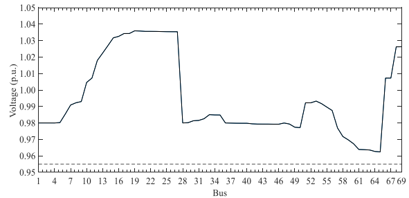
Fig. 16. The voltage profile case 2: distribution system with PV 5 units.
